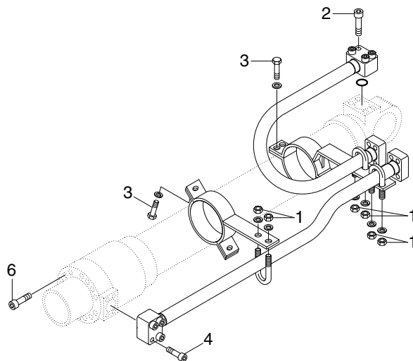
ARM CYLINDER
